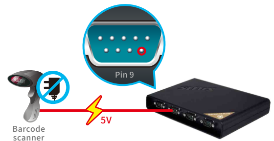
1-4 SUNIX Patented Powered COM Design
